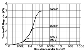
Typical Terminal Voltage Characteristics
